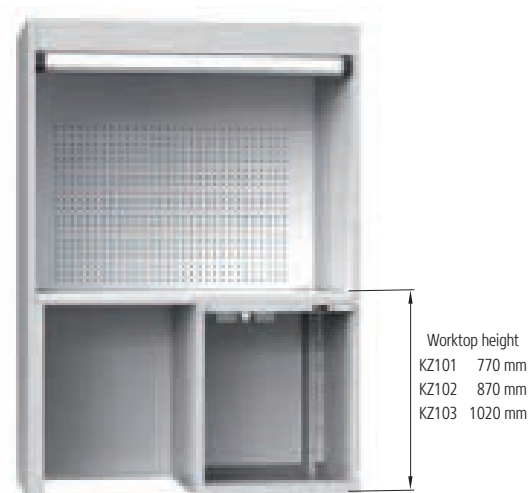
Control workst. body, width 1462 mm with leg 36 x 36D
